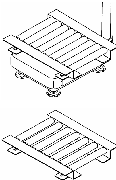
Figure 4 Conveyor load receptor
